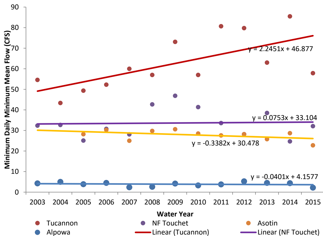
Figure 8: Minimum daily mean flow (cfs) by water year for the Tucannon River at Marengo, North Fork Touchet above Dayton, Asotin Creek above George Creek and Alpowa Mouth. Trend line and slope provided for each watershed over the period of record. Data provided by Washington Department of Ecology ( https://fortress.wa.gov/ecy/eap/flows/station.asp?wria=35 ).
