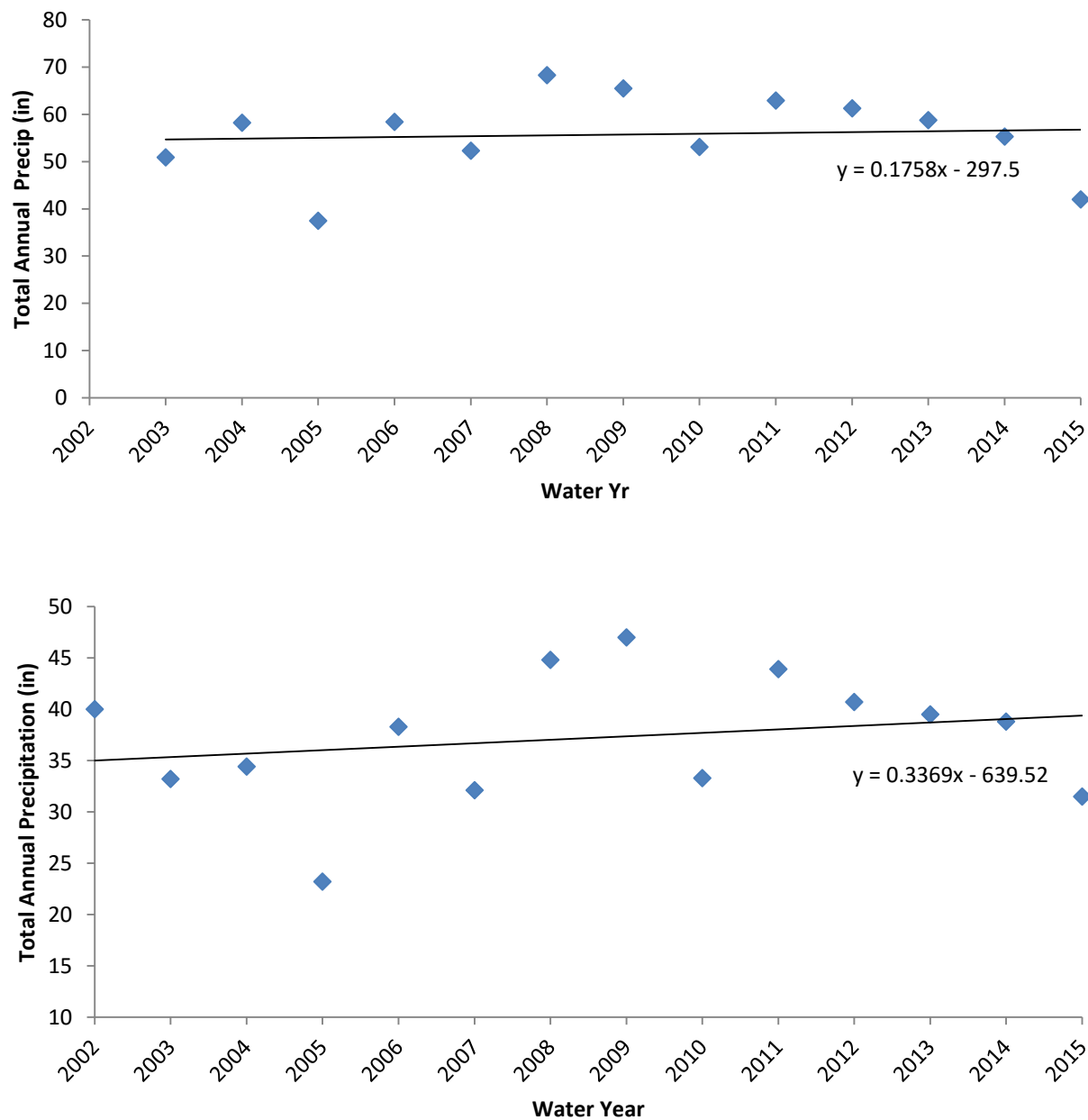
Figure 7: Total annual precipitation measured at the NRCS SNOTEL gage for the period of record at the Touchet (upper) and Spruce Springs (lower) gages. The Touchet gage is located near the Tucannon basin and the Spruce Springs gage is located south eastern most part of the Tucannon Basin.
