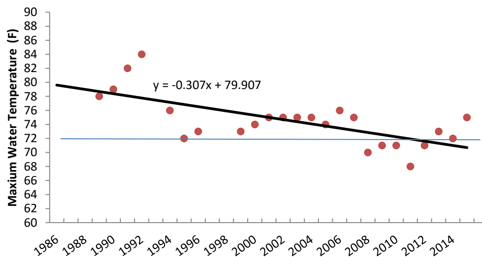
Figure 4: Mean daily maximum stream temperature measured at the Tucannon River Washington Department of Ecology Marengo gage between 2003 to present. The time periods prior to 2003 was collected near Marengo by WDFW monitoring. The fine horizontal line indicated the recovery objective of <4 days greater than 72°F annually. Data provided by Washington Department of Ecology ( https://fortress.wa.gov/ecy/eap/flows/station.asp?wria=35 ).
