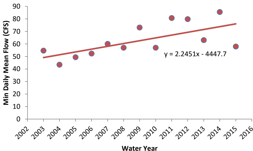
Figure 6: Minimum daily mean flow measured at the Tucannon River Marengo stream gage from 2002 through 2015 water year. Data provided by Washington Department of Ecology ( https://fortress.wa.gov/ecy/eap/flows/station.asp?wria=35 ).
